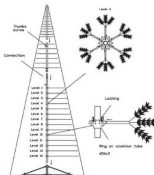
V 500 steel mast structure
